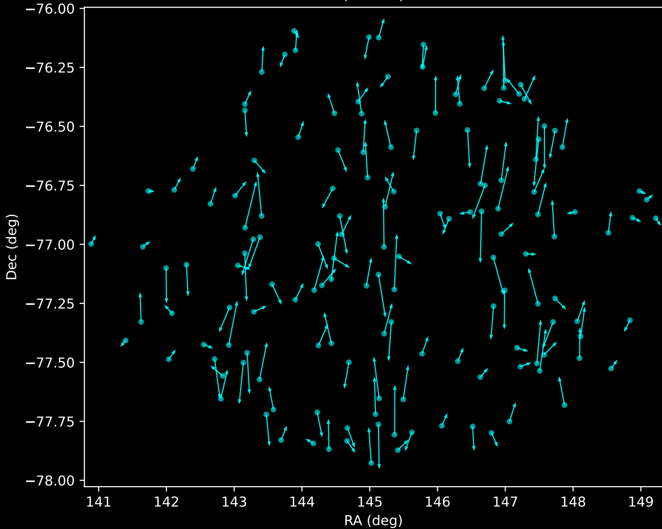
GALAH DR4 Noise Stream Proper Motion Vectors (n=147)
