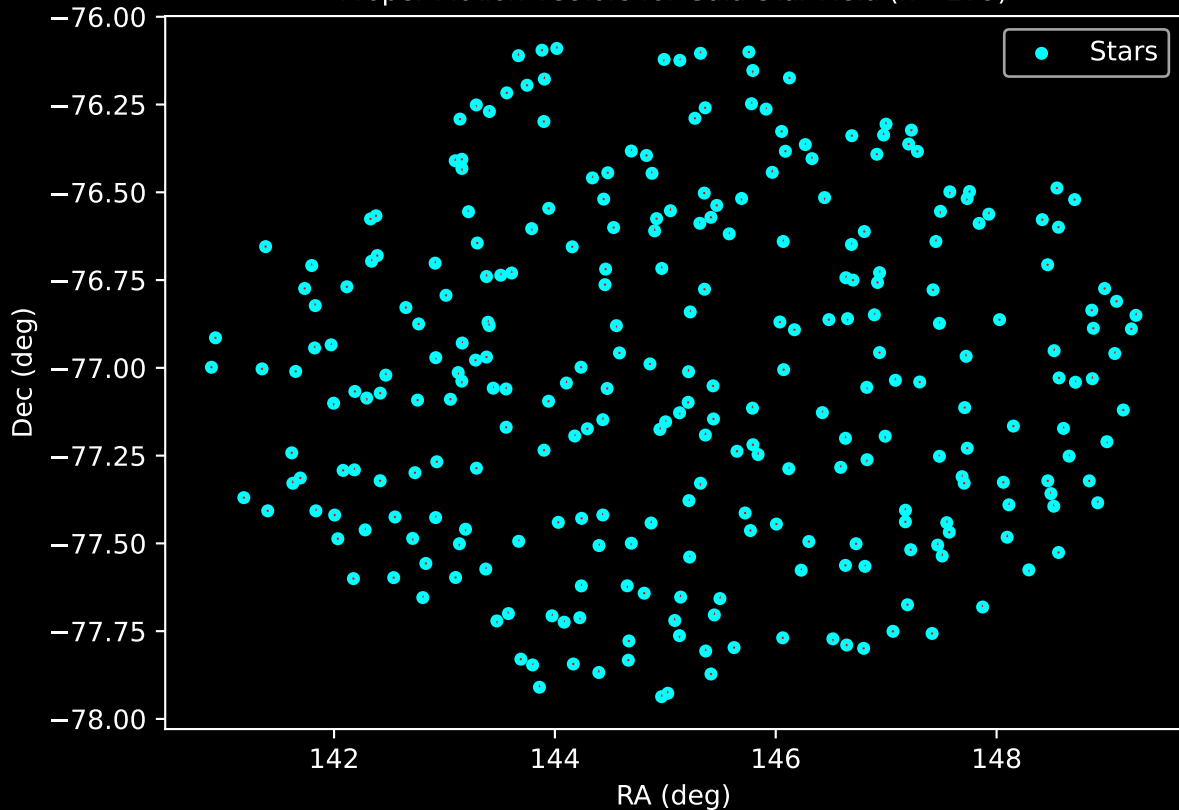
GALAH DR4 Field: [315] Proper Motion Vectors for Gaia Star Field (n= 279)
