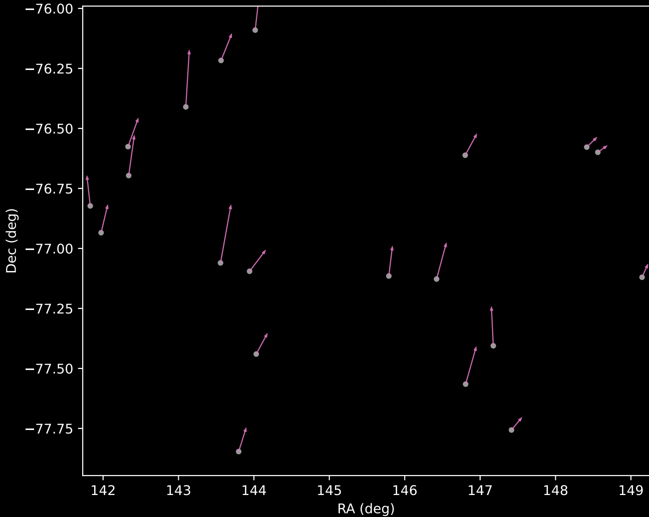
GALAH DR4 Cluster 12 Proper Motion Vectors (n=20)
