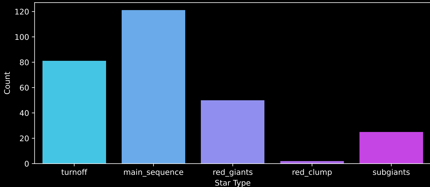
GALAH DR4 Field: [315] Count plot of Star Type
