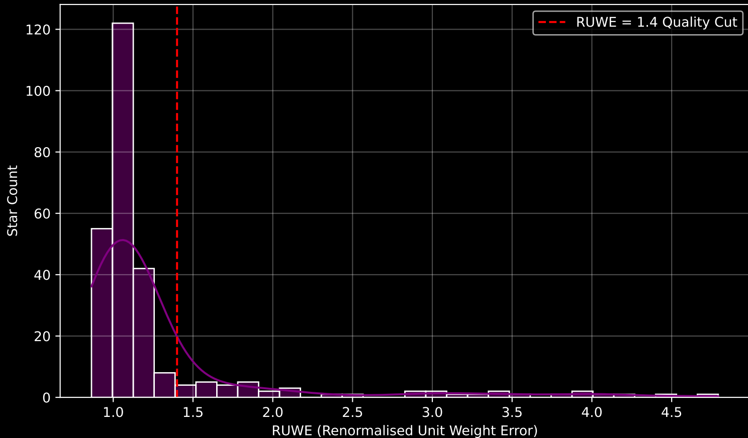
GALAH DR4 Field [315] RUWE Distribution (n= 268)
